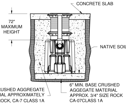
EXCAVATION AND BACKFILL DETAIL (INTERIOR OR EXTERIOR)
